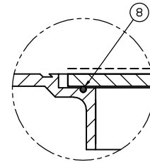
VIEW A ENLARGED SECTION OF NEOPRENE CUSHION
