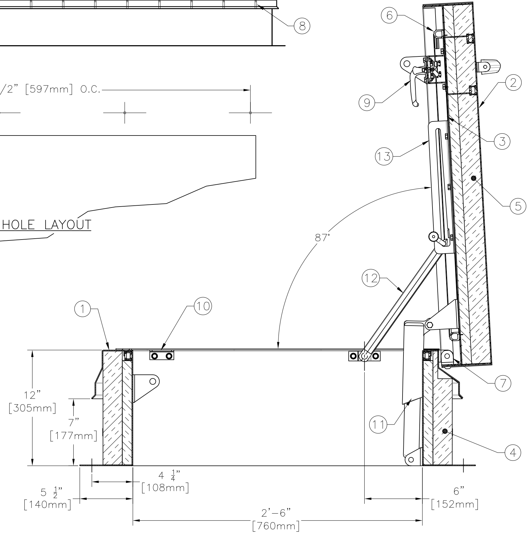
SECTION
